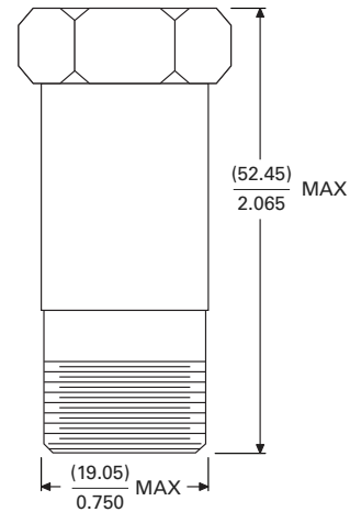
MS33678-10SL-3P (SPDT) IS33678-10SL-4P (SPST NC/NO)
